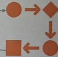
Stream Processing
